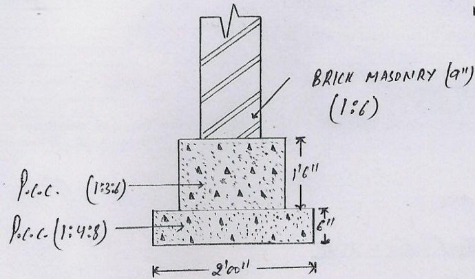
FIG. 2 → FOUNDATION DETAILS
